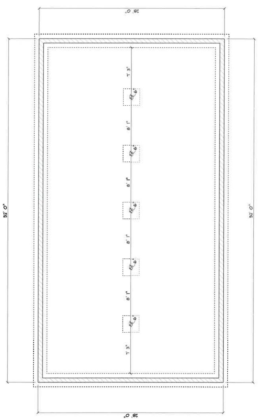
FOUNDATION SCALE: 1/4" = 1'-0"
